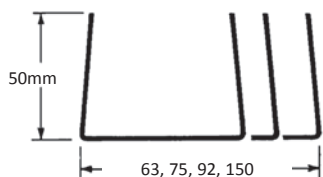
DEFLECTION HEAD TRACK SIZES
